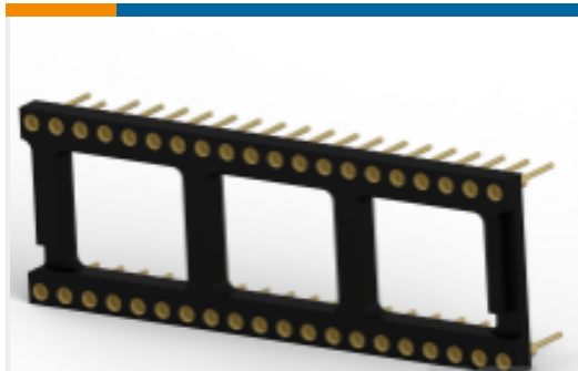
TE Part # 2-1571586-9 DIP Socket: Standard, Screw Machine, Open, Gold
