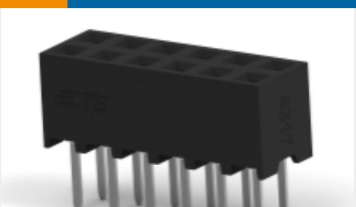
TE Part # 1-2314824-2 12P,2MM,B-B,REC,DRV,T,2.7,0.1AU,TB, W/CAP
