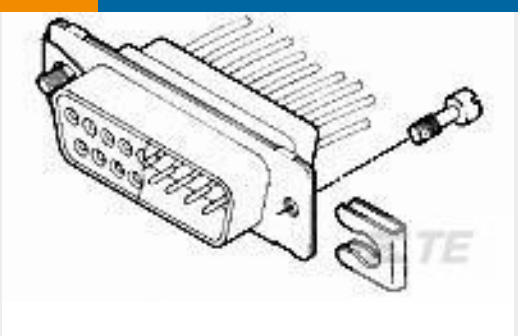
TE Part # 5745136-3 SCREW RETAINER KIT
