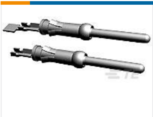
TE Part # 66566-1 III+ PIN,24-20,30AU>10,LP
