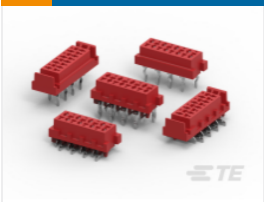
TE Part # 215079-6 Female-on-Board Connector, Top Entry
