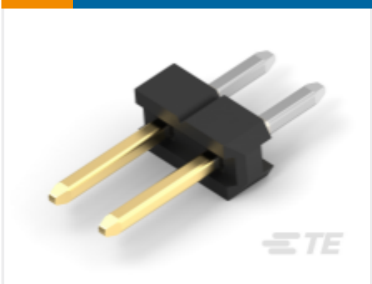
TE Part # 2355045-2 2P,2MM,BRK HDR,SRVT,2.8,0.1AU,TB
