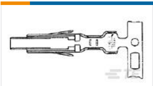
TE Part # 2-1703494-1 3POS, MCON 1.2 LL TAB SEALED COD B
