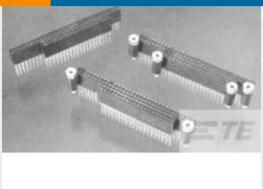
TE Part # 1375795-1 ASSY, 64/40 POS PC104
