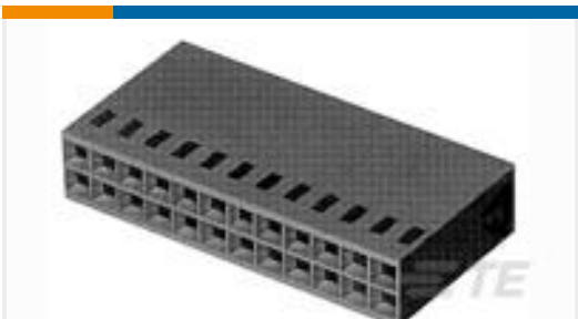
TE Part # 87456-7 12 MODIV HSG COMP DR .100CL
