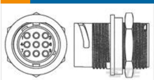
TE Part # 1445823-3 REC,11-6,FLNG MT,LG INS,STD KE
