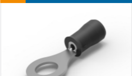
TE Part # 51863-4 PIDG Ring Tongue Terminals
