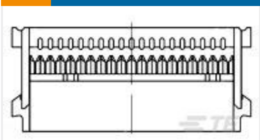
TE Part # 1658526-9 609-1441LF FEM SOCKET,LEAD FREE
