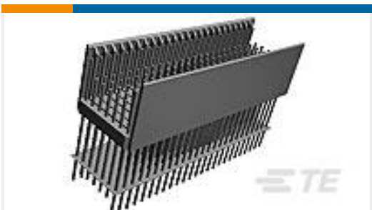
TE Part # 5100141-4 2MM H.M. TYPE "B" PIN ASSY.
