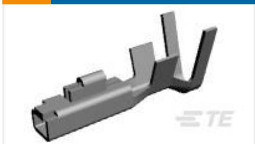
TE Part # 175156-2 U/P REC CONT L/P
