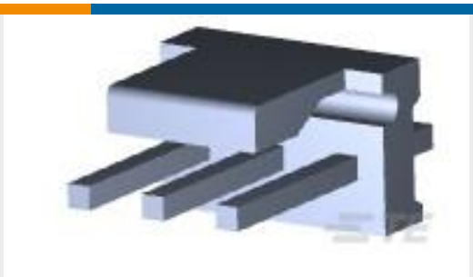
TE Part # 3-641208-3 03P MTA156 HDR ASSY FL ST LF
