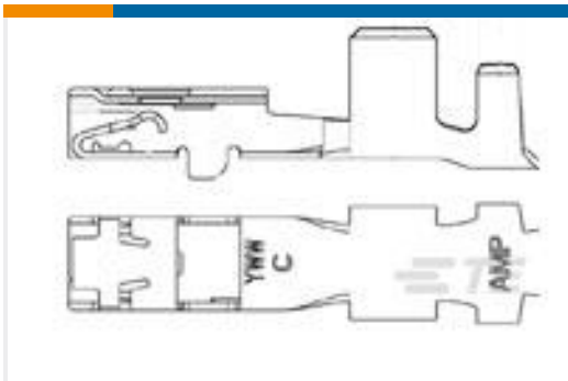
TE Part # 1326030-1 2.8MM RECP,UNSEAL,22AWG
