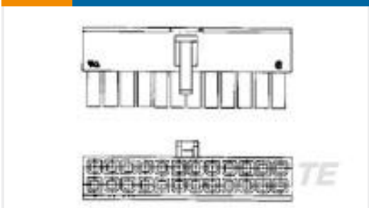
TE Part # 182922-1 CPC SQ.FL.RCPT STD SEX
