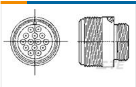
TE Part # 213650-1 CPC 20-14 FREE HANGING RCPT
