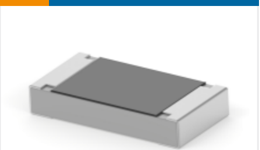
TE Part # 4-2176344-3 CRGCQ 1206 10M 5%
