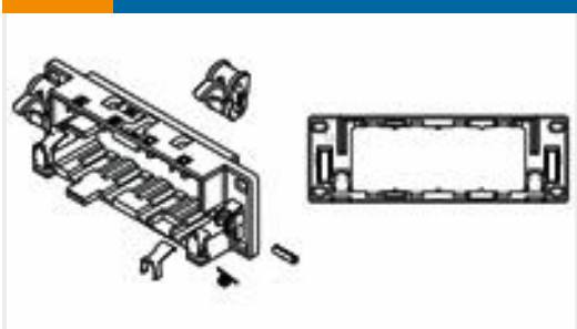
TE Part # 2069526-1 DYNAMIC FRAME PANEL W key
