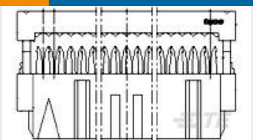
TE Part # 5-215882-0 50 WAY GREY MK II RECEP
