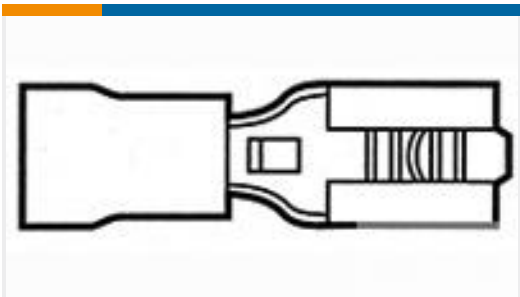
TE Part # 184235-1 RECEPT,PIDG FASTON 16-14 187
