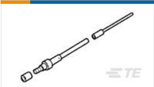
TE Part # 226782-2 ARINC SIZE 15 SOCKET
