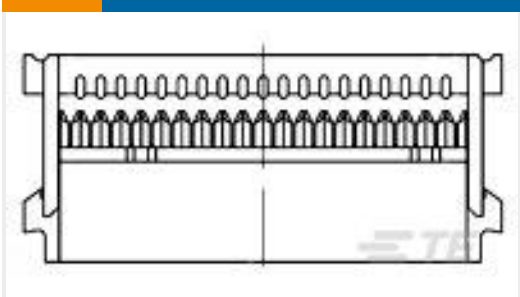
TE Part # 1658526-1 609-0630LF FEM SOCKET,LEAD FREE
