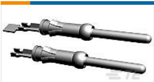
TE Part # 66099-1 III+ PIN,18-16,30AU>10,LP
