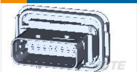
TE Part # 3-1564526-1 18POS,TAB 1.6X0.6,TAB HSG,ASSY
