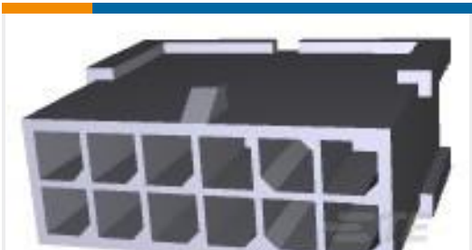
TE Part # 1-794616-2 FREE HANG DBL ROW HSG 12 POS
