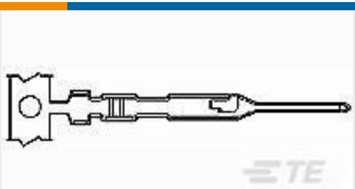
TE Part # 5-104506-6 MTE PIN 28-32 AWG PLTD
