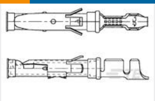
TE Part # 163088-1 062 SOC.ASS. TYP3+
