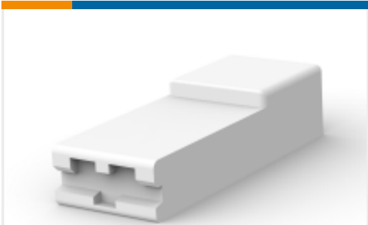
TE Part # 926539-1 250 FASTON HSG. REC. 1P NATURAL
