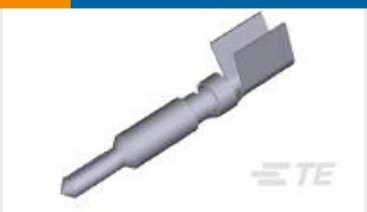
TE Part # 770246-3 UMNL II PIN PTPPHBZ LP 12-10
