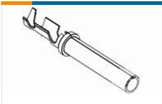
TE Part # 776492-2 SOC, SF, SIZE 16, 14-18 AWG, NI/SN
