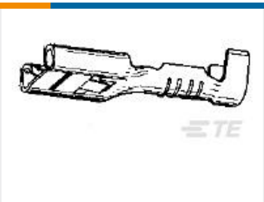
TE Part # 735222-1 FF 250 REC 1.0-2.5 MM2 0.32X19.30 BR
