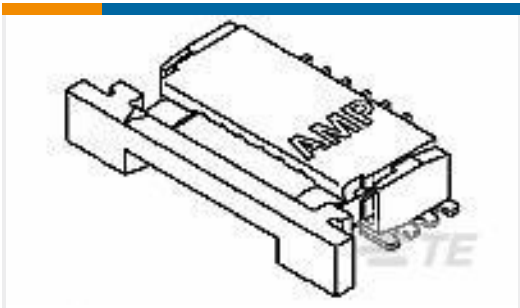
TE Part # 84952-5 1MM FPC HORZ.BTTM CONT.ASS.5P
