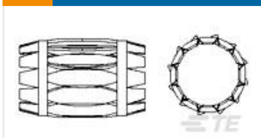
TE Part # 205690-2 SOC. BLOCK 28 POS. SPL.
