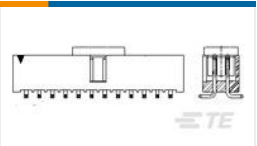
TE Part # 4-1775144-4 BOX HDR 2.0 PTH VT DR 44 POST
