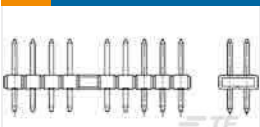
TE Part # 2-5178751-1 AMPMODU 2MM HDR V-TYPE ASSY
