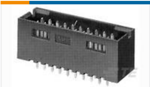
TE Part # 5-102619-1 06 MODII HDR DRST SHRD .100CL
