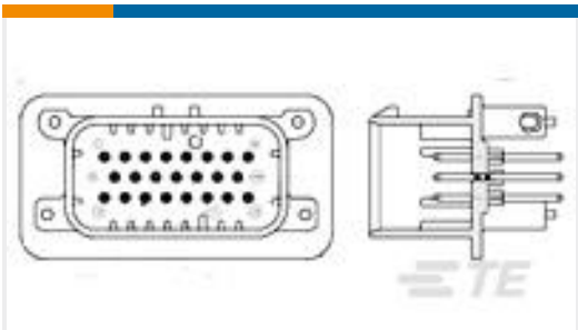
TE Part #776230-1 35POS,PIN DIA 1.3,HDR ASSY, 180DEG,COD 1
