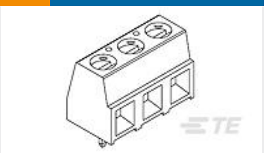
TE Part # 1776118-3 3P TERM-BLOK,PCB,HIGH TEMP
