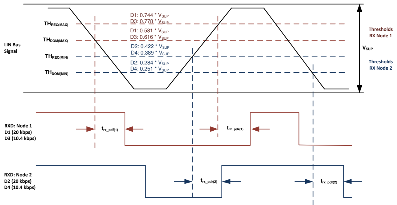
Figure 6-13. Propagation Delay
