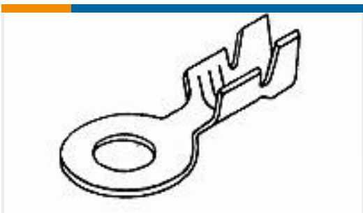
TE Part # 640007-3 RING TERMINAL 16-14 AWG TPBR
