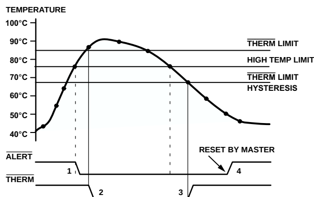
Figure 83. \overline{THERM} Behavior
