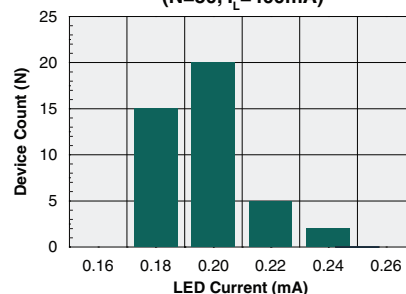
Typical I_F for Switch Dropout (N=50, I_L=400\text{mA} )
