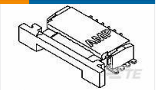
TE Part # 2-84952-8 1MM FPC HORZ.BOTTOM CONT. ASSY 28P
