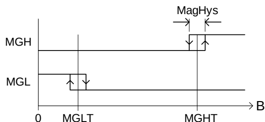
Figure 28: MGH and MGL Signals as a Function of the Field Strength
