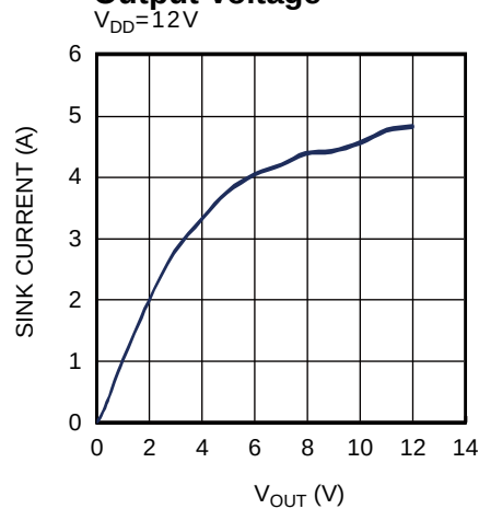
Sink Current vs. Output Voltage V_{DD} = 12V
