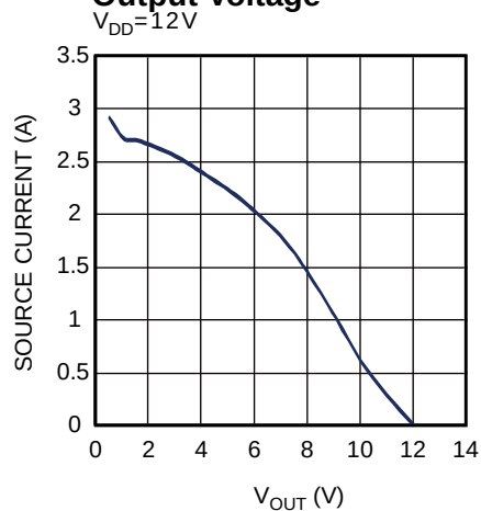
Source Current vs. Output Voltage V_{DD} = 12V
