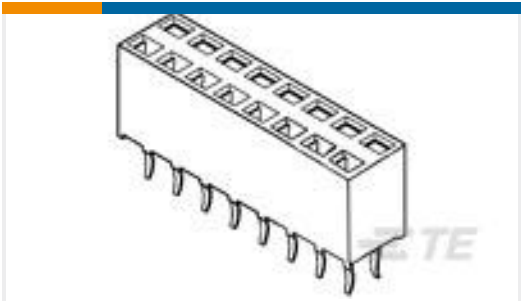
TE Part # 215309-9 2X9P HV100 REC CON. TE, 8.5MM
