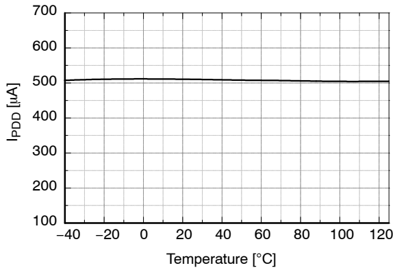
Figure 16. Operating V_{DD} Supply Current vs. Temperature
