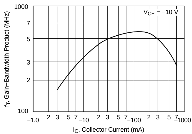
Figure 9. f_T - I_C
