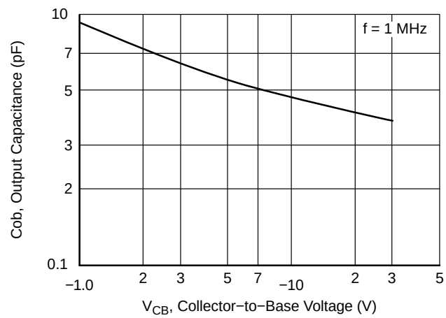
Figure 8. C_{ob} - V_{CB}
