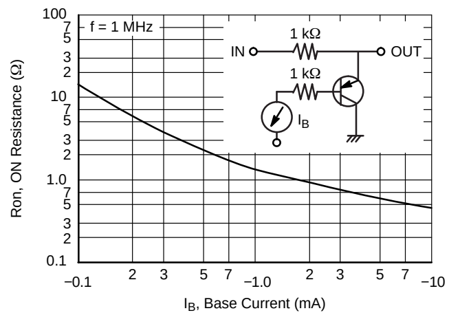
Figure 10. R_{on} - I_B
