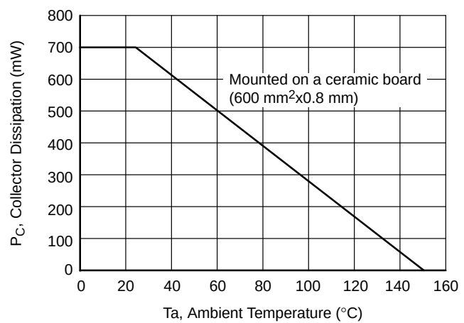
Figure 11. P_C - T_a
