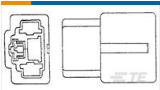
TE Part # 176773-5 FF 250 CAP HSG 3P NYLON NAT
