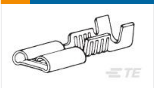
TE Part # 42781-2 205 FASTON REC 18-14 AWG TPBR
