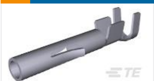
TE Part # 350536-2 UMNL SOK 20-14 .0126 AUNI/BR
