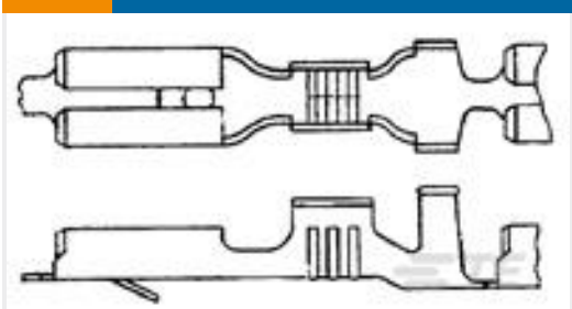
TE Part # 170015-1 FF 110 REC 20-16AWG BR
